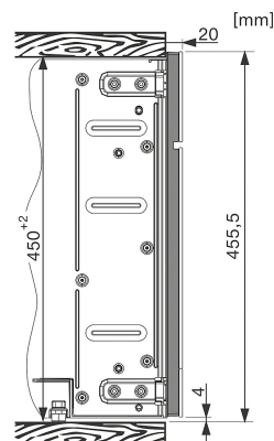
CVA5060, CVA5065, CVA6401, CVA6405, CVA6800, CVA6805, side view (installation drawings)
