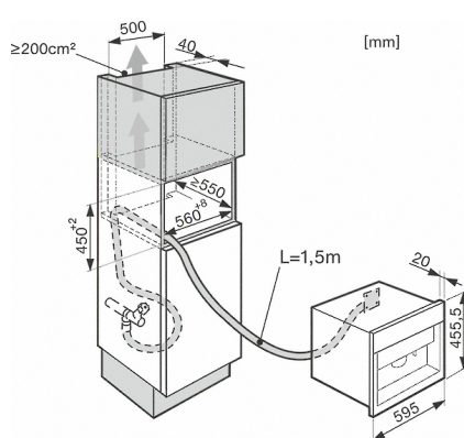
CVA5065, CVA6405, CVA6805, plumbed in water supply (installation drawings)
