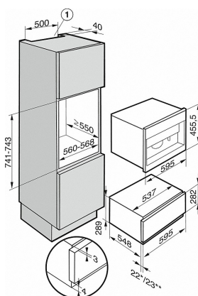
ESW 6129, ESW 6229 (Installation drawing)
